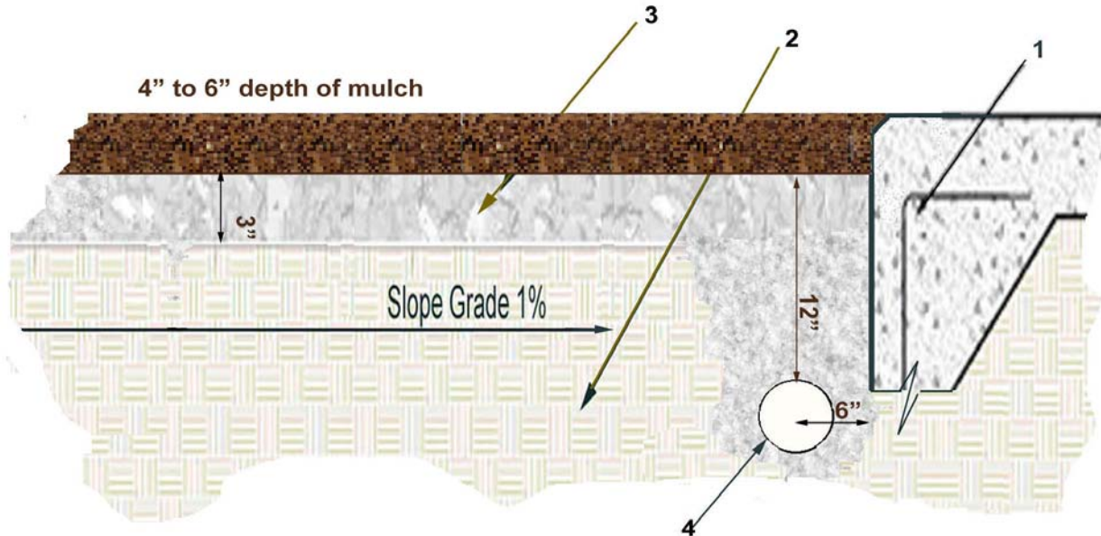
PolyStar “Tumble Tot” Rubber Mulch Loose or Poured-in-Place Playground System Detail
